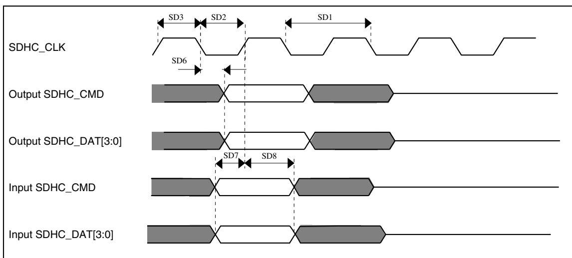
Figure 36. SDHC timing
